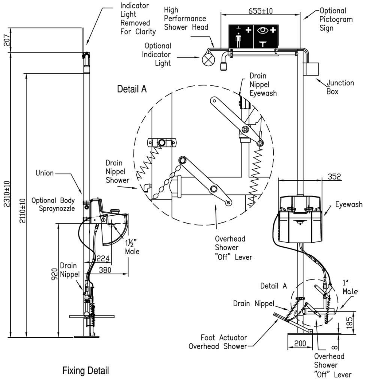
Front Elevation
