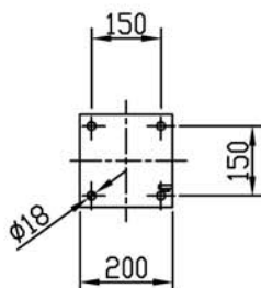
Fixing Detail
